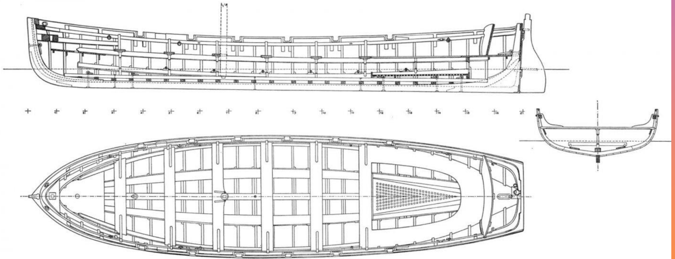
Inboard profile reveals solid construction with hull reinforced by abundance of angle-brackets and knees.
